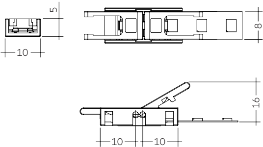
ACL connector PCB-PCB
