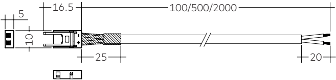
ACL connector Wire-PCB
