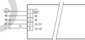
switchDIM PCA T8 EXCEL one4all Ip xtec
