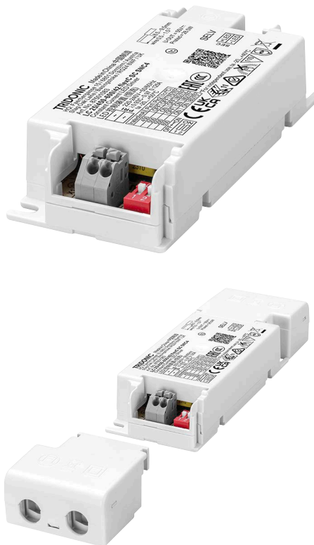
With strain-relief (see accessory)
