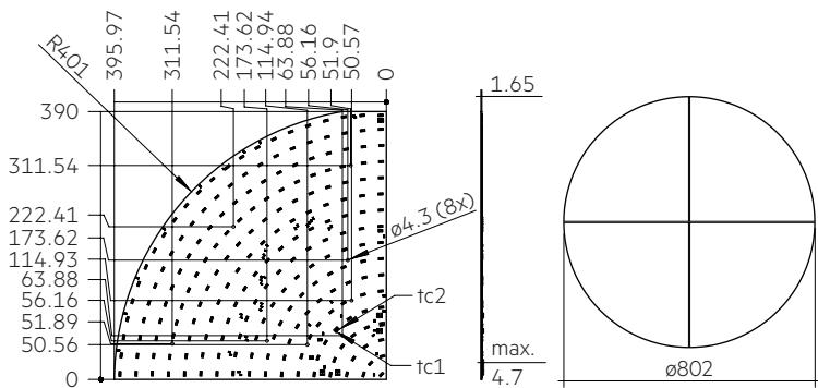
CLE 401mm 2450lm 927-965 4T PRE2
