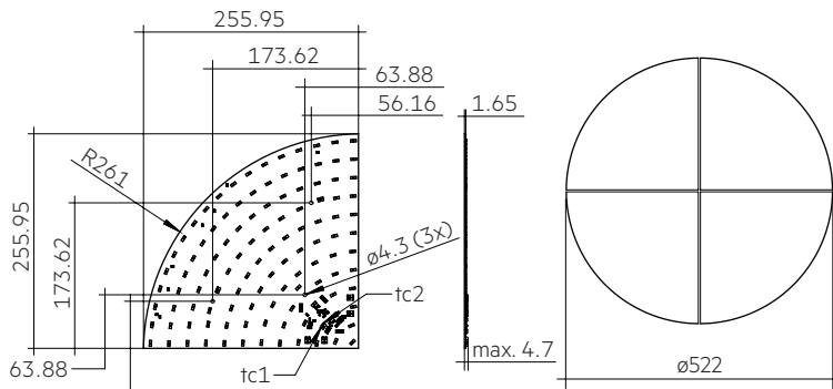
CLE 261mm 4600lm 927-965 4T PRE2
