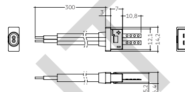
ACL plug connector Wire-PCB IP67 left
