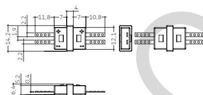
ACL plug interconnector IP67
