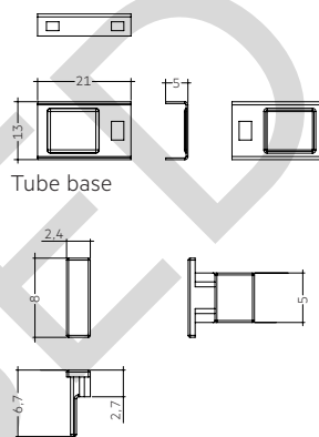
Tube base Plug
