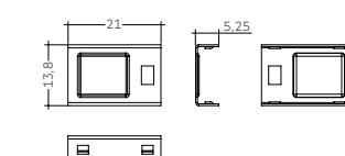
Tube cover
