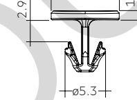
ACL CLIP 4.3mm PUSH-FIX Long
