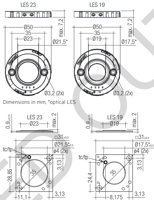
Dimensions in mm, *optical LES
