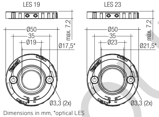
Dimensions in mm, *optical LES
