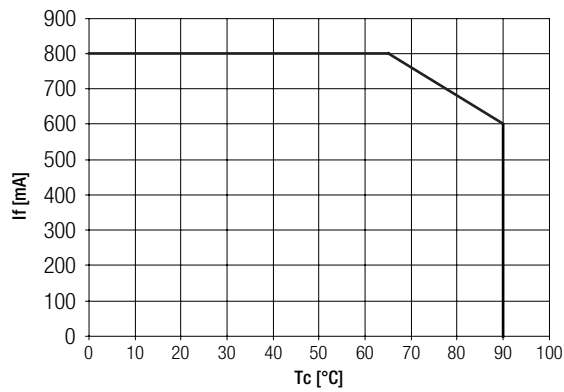
Derating curve for TALEX(module STARK SLE PURE G3 10 CLASSIC 4,000 K
