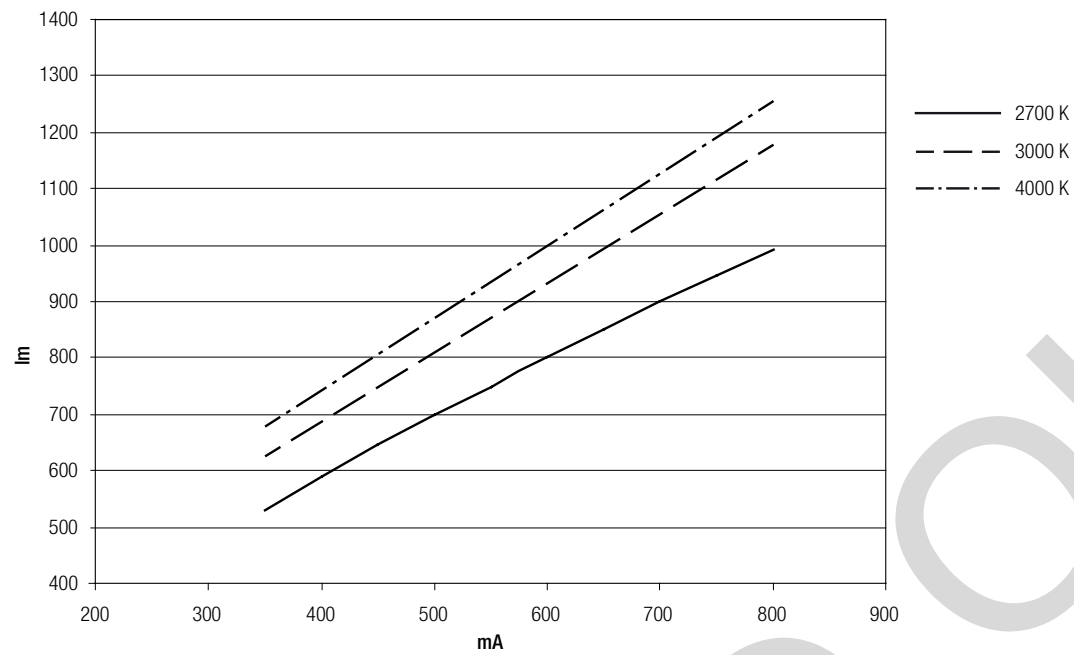
Luminous flux and operating current for TALEX module STARK SLE PURE G3 10 CLASSIC at t_p = 65^\circ\text{C}
