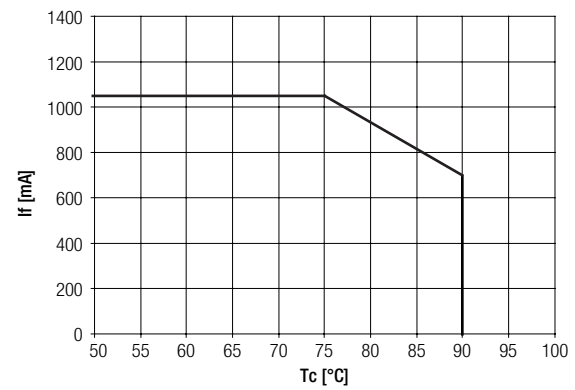
Derating curve for TALEX(module STARK SLE PURE G3 17 CLASSIC 4,000 K
