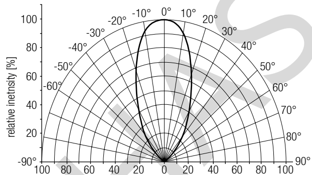
DLA G1 100mm 1000lm 8xx xxx SNC with 60° reflector
