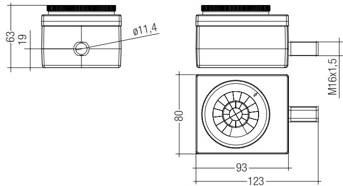
ACU MOUNTING BOX 16DPI HIGHBAY ACU MOUNTING BOX 16DPI HIGHBAY with sensor
